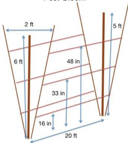
California V-Trellis (with wooden posts) Post-Bloom
